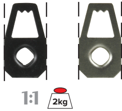
1-Hole Hangers
