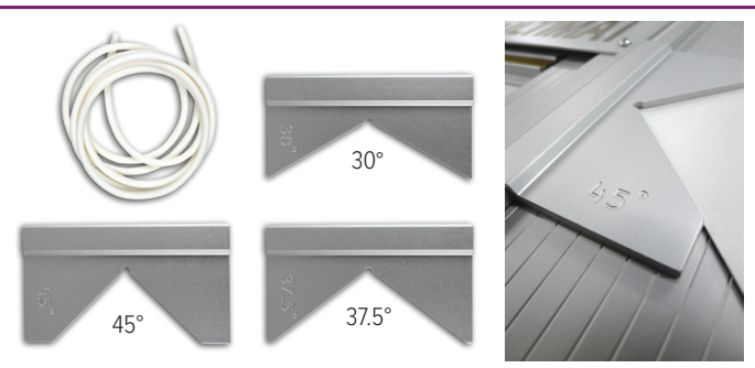
Multi-Angle Cutting Gauges shown on an Ultimat Gold
